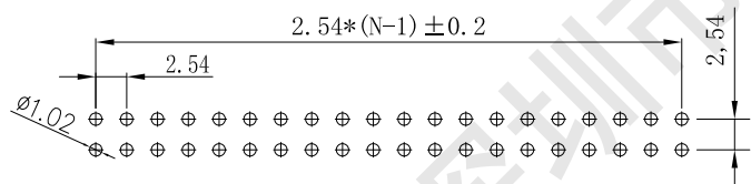
PCB LAYOUT
