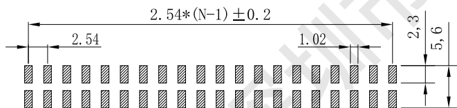
PCB LAYOUT
