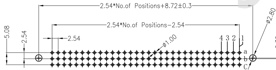
PCB LAYOUT(RECOMMENDED) (TOP VIEW TOL. : ±0.05)
