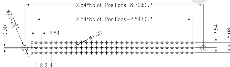
PCB LAYOUT(RECOMMENDED) (TOP VIEW TOL. :±0.05)
