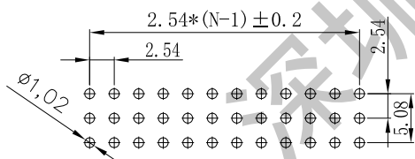
PCB LAYOUT
